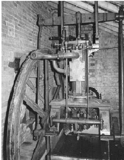
A steam engine to work the mill when the pond has dried up.
