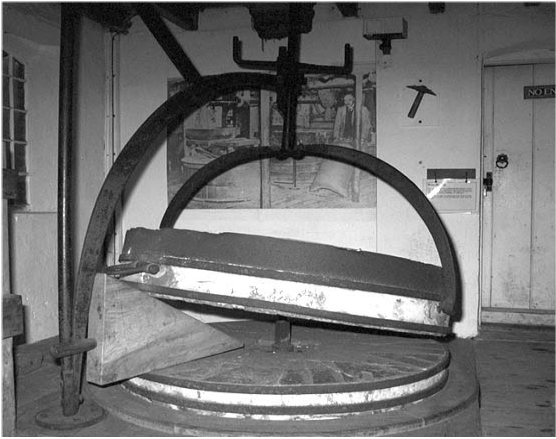
A jack to lift up the mill stones.
